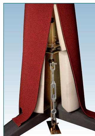
tension system
